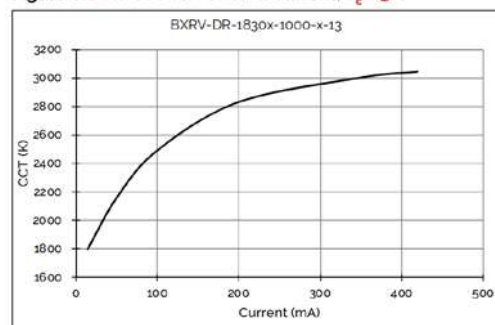
Figure 8: 12W CCT vs. Forward Current, T_c = 25^\circ\text{C}
