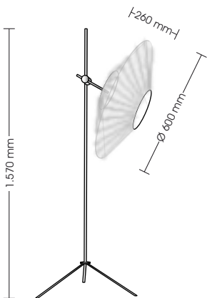
56663-60 230V 1x E27 LED
