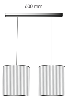
56563-2-20 230V 2x E27 LED
