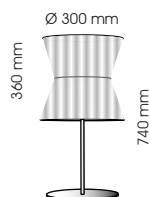
56712-30 230V 1x E27 LED
